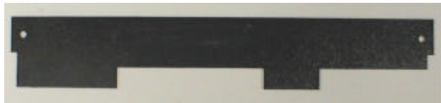
801,810,53x.x1 Anti-Nose Diving Shim 3 1/4" H x 19 5/8" L x .093" T
